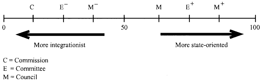
FIGURE 1. Sample arrangement of ideal points and qualified majorities
