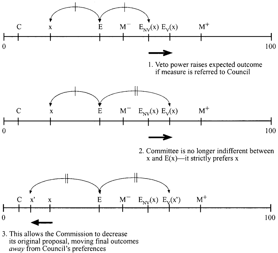
FIGURE 4. Change in equilibrium with Council veto
